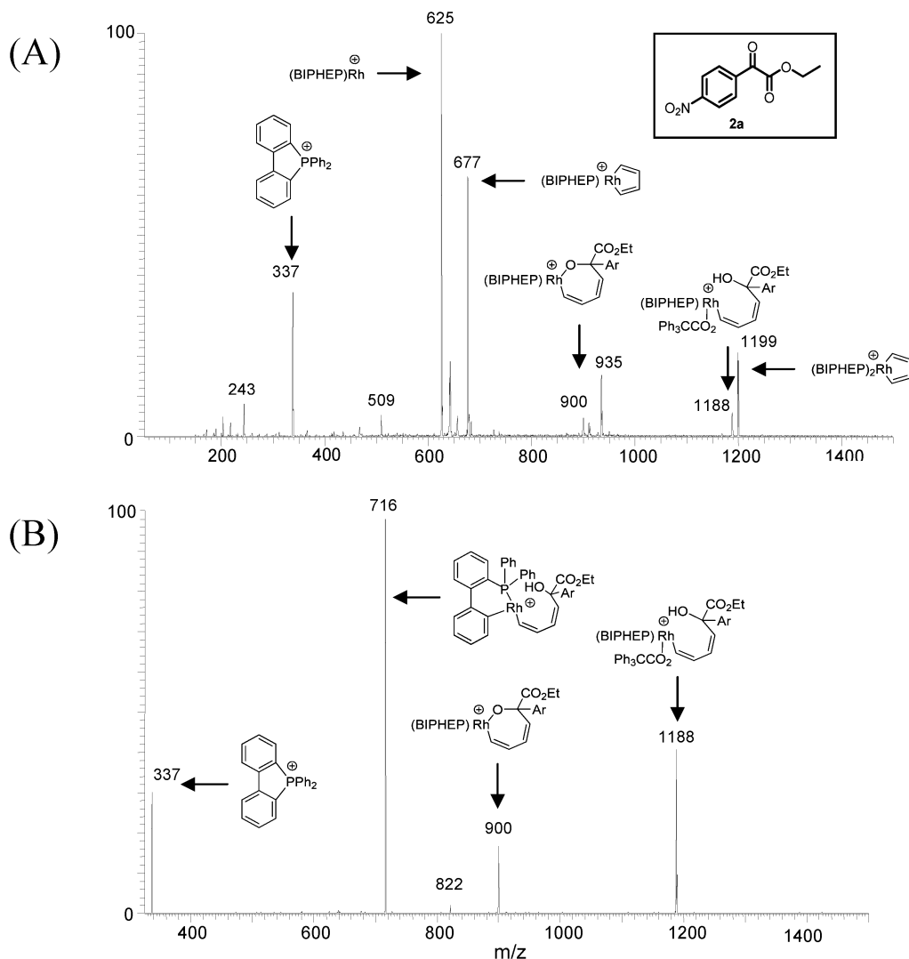
Figure 1. Hydrogen-mediated coupling of gaseous acetylene to \alpha -ketoester 2a ( Ar = p\text{-NO}_2\text{Ph} ) using triphenylacetic acid as cocatalyst. (A) ESI mass spectrum with proposed structural assignment of observed ions. (B): CAD mass spectrum of the ion of m/z 1188 with proposed structural assignment of observed ions.
