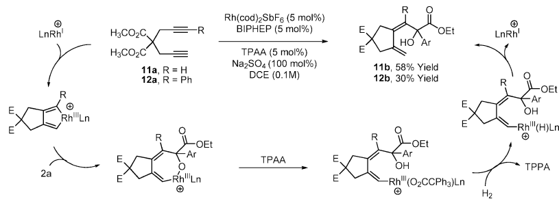
Scheme 2. Proposed Catalytic Mechanism for the Hydrogen-Mediated of 1,6-Diynes 11a and 12a to \alpha -Ketoester 2a Using Triphenylacetic Acid As Cocatalyst
