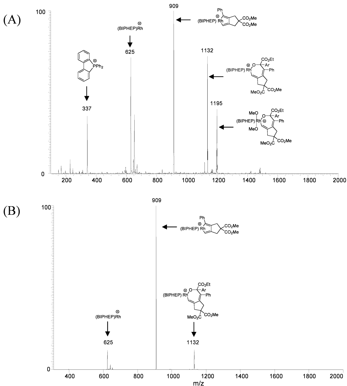
Figure 5. Hydrogen-mediated of 1,6-diyne 12a to \alpha -ketoester 2a ( \text{Ar} = p\text{-NO}_2\text{Ph} ) using triphenylacetic acid as cocatalyst. (A) ESI mass spectrum with proposed structural assignment of observed ions. (B) CAD mass spectrum of the ion of m/z 1132 with proposed structural assignment of observed ions.
